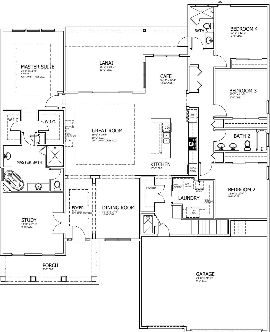
FIRST FLOOR
